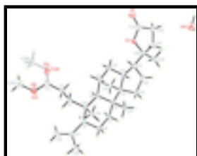
Fig. 1. The molecular structure of the title compound, with 40% probability displacement ellipsoids and the atom-numbering scheme. Open bonds show the minor component.
