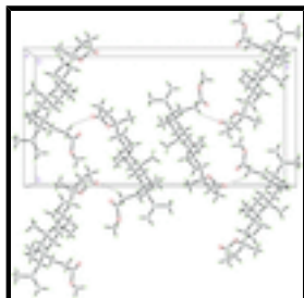
Fig. 2. The crystal packing of the major component of the title compound viewed along the a axis, showing screw chains along the [010] direction. Weak C—H...O interactions are shown as dashed lines. Water molecules and atoms of the minor disorder component were omitted for clarity.
